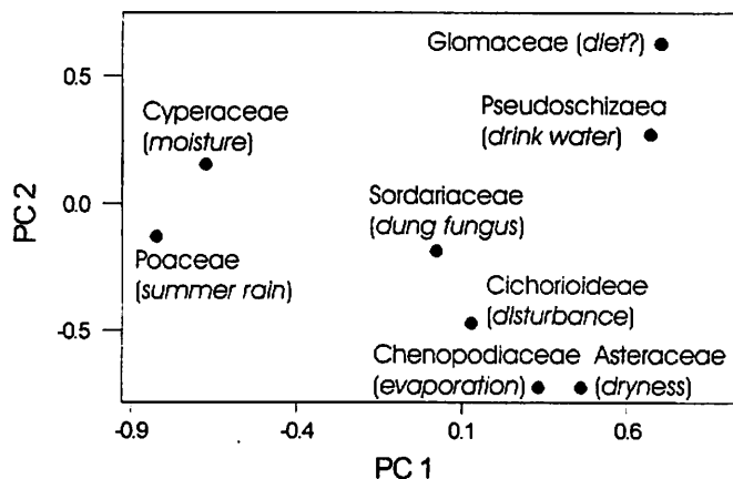
Fig. 11. First and 2nd principal component values of a single data matrix of the most prominent pollen and microfossil types of both study areas as illustrated in Figs. 4-7. Possible environmental indications or origin of these palynomorphs are suggested in italics
