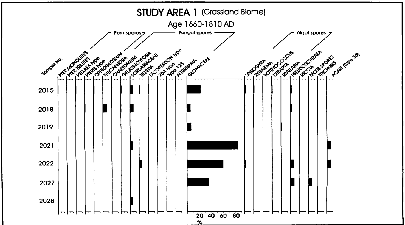
Fig. 5. Spores and other palynomorph percentages in fossil cow dung samples from Study Area 1
